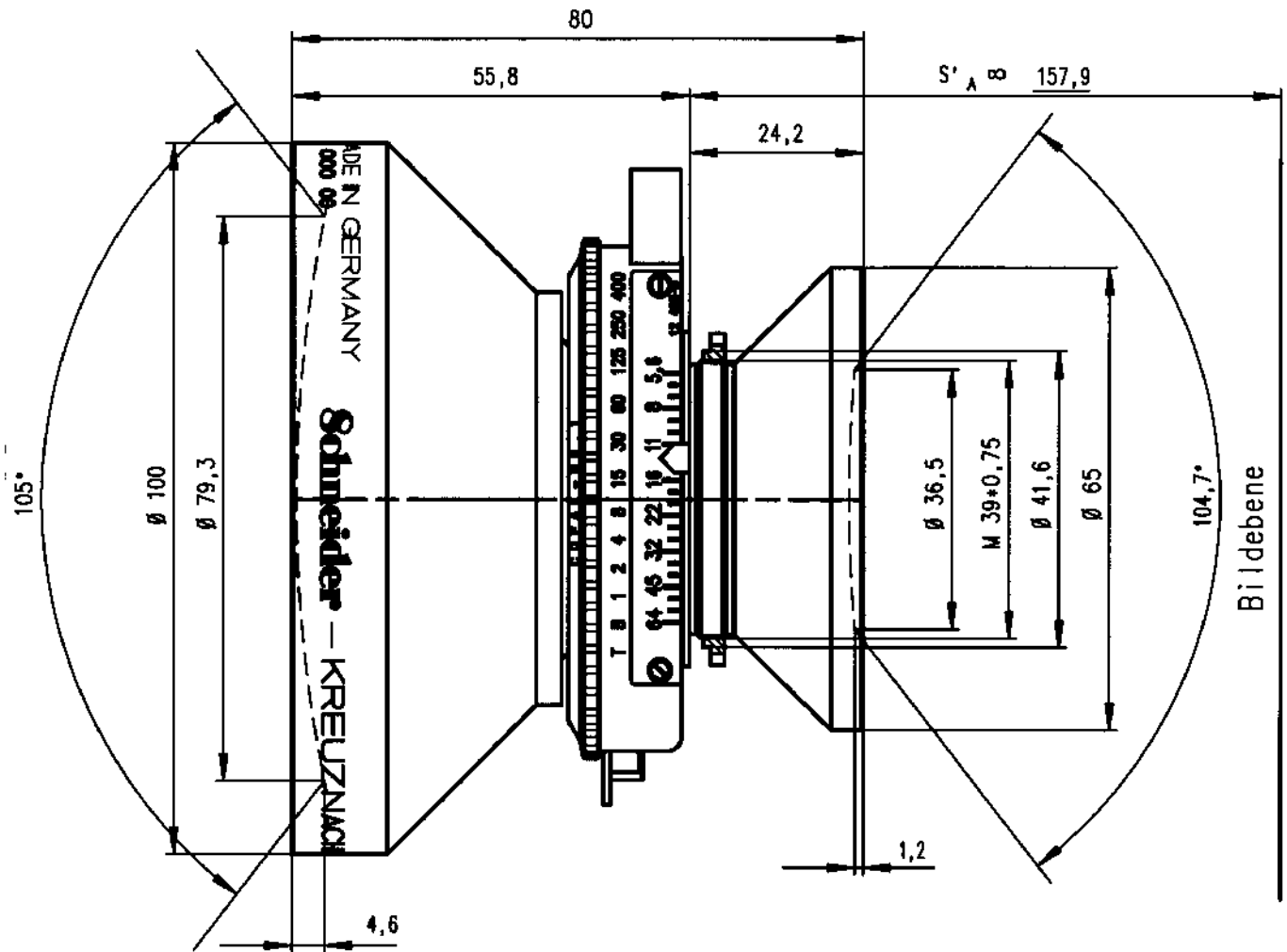
SUPER-SYMMAR 5,6/150 XL-105° ASPHERIC in Copal 1
